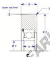
Insert Bearing
