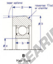
Style VII : Chamfer of reverse Fillet
