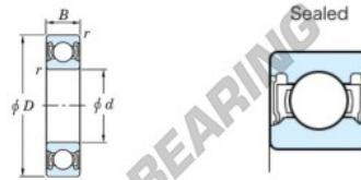
Boundary dimensions
