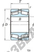
Boundary dimensions
