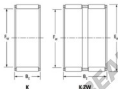
Ball or needle roller and cage assemblies
