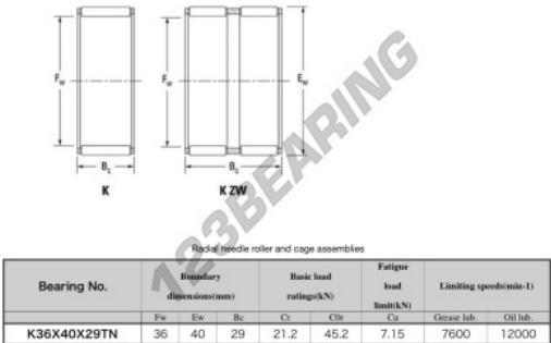
Boundary dimensions
