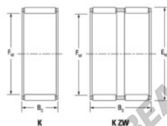
Radial inside roller and cage assemblies
