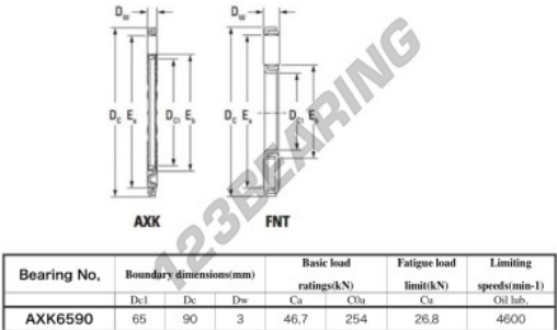
Boundary dimensions
